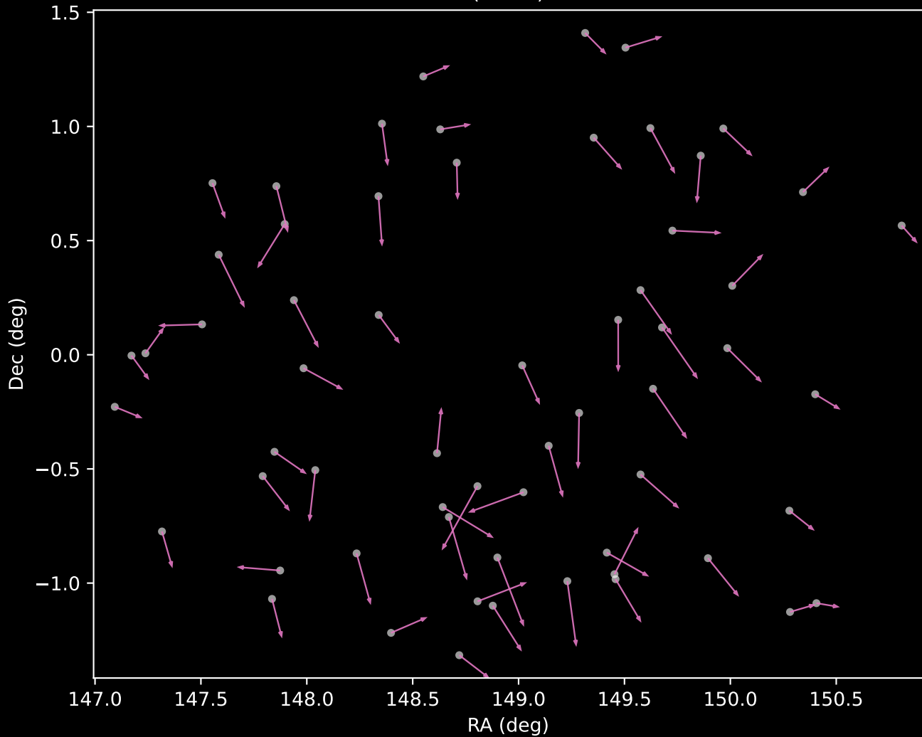
APOGEE DR17 Cluster 12 Proper Motion Vectors (n=61)
