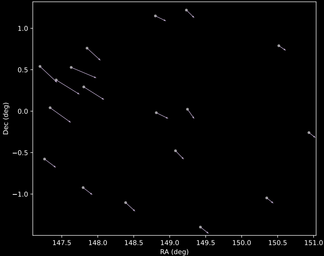
APOGEE DR17 Cluster 9 Proper Motion Vectors (n=18)
