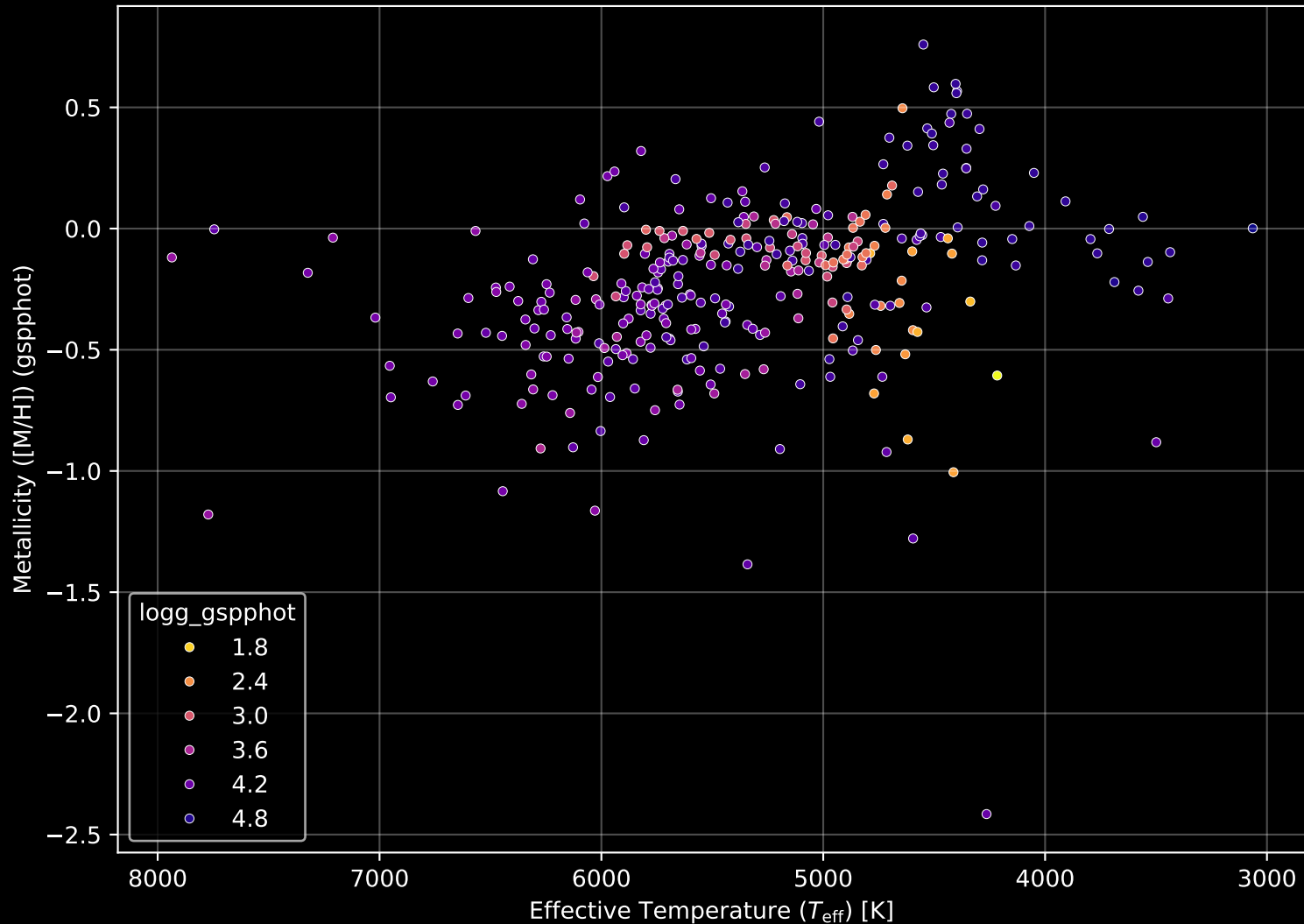
APOGEE DR17 Field: [181-46_MGA] Stellar Population Parameters (n= 326)
