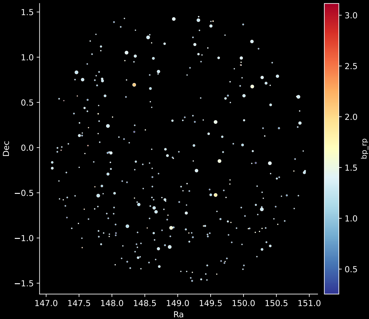
APOGEE DR17 Field: [181-46_MGA] Stars: 326
