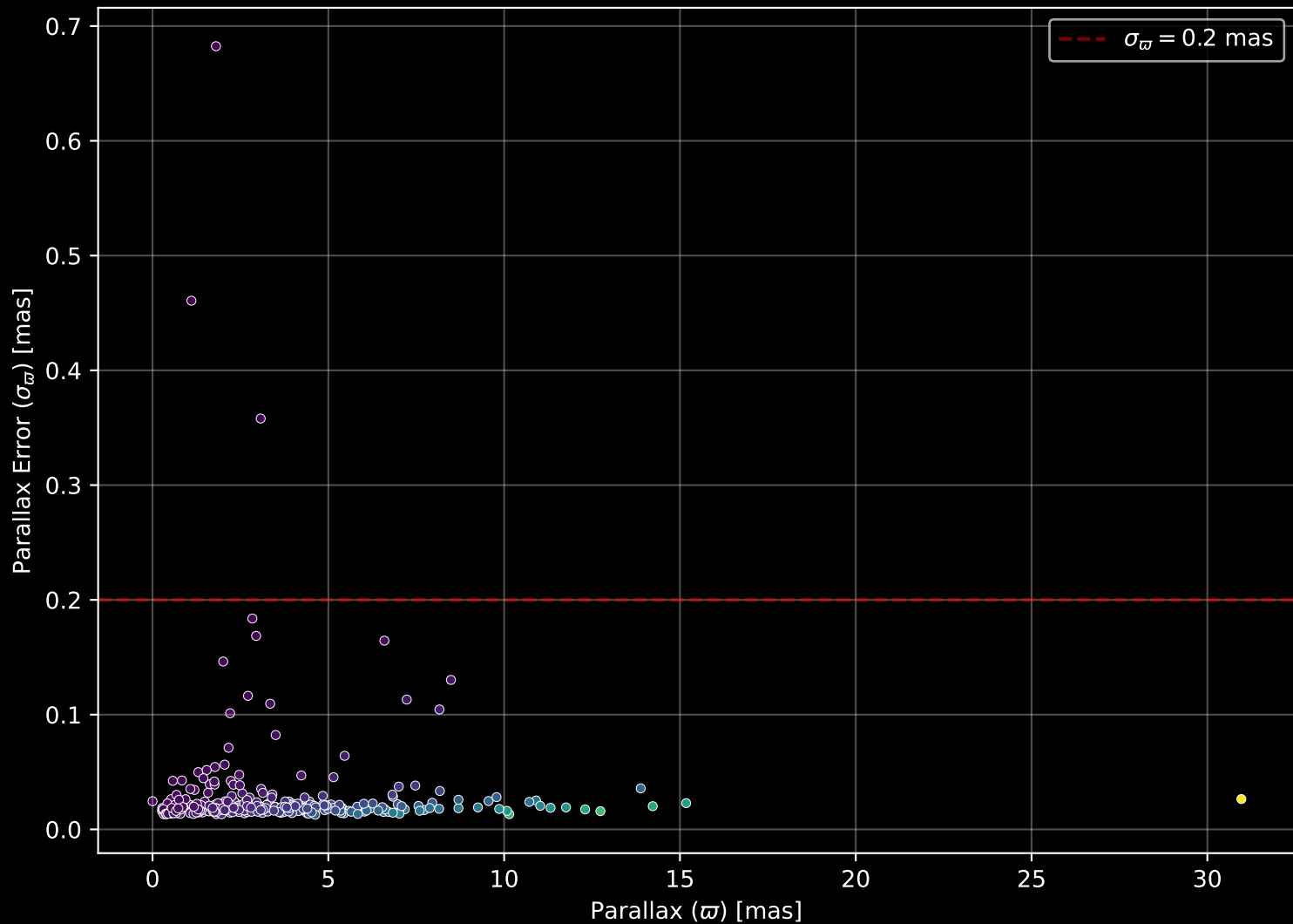
APOGEE DR17 Field: [181-46_MGA] Parallax Quality (n= 326)
