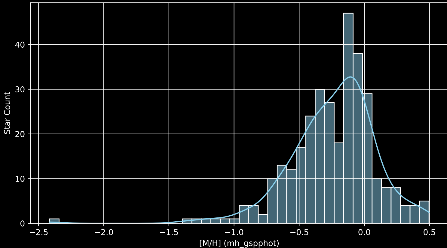
APOGEE DR17 Field: [181-46_MGA [M/H] (mh_gspphot) (n= 321)
