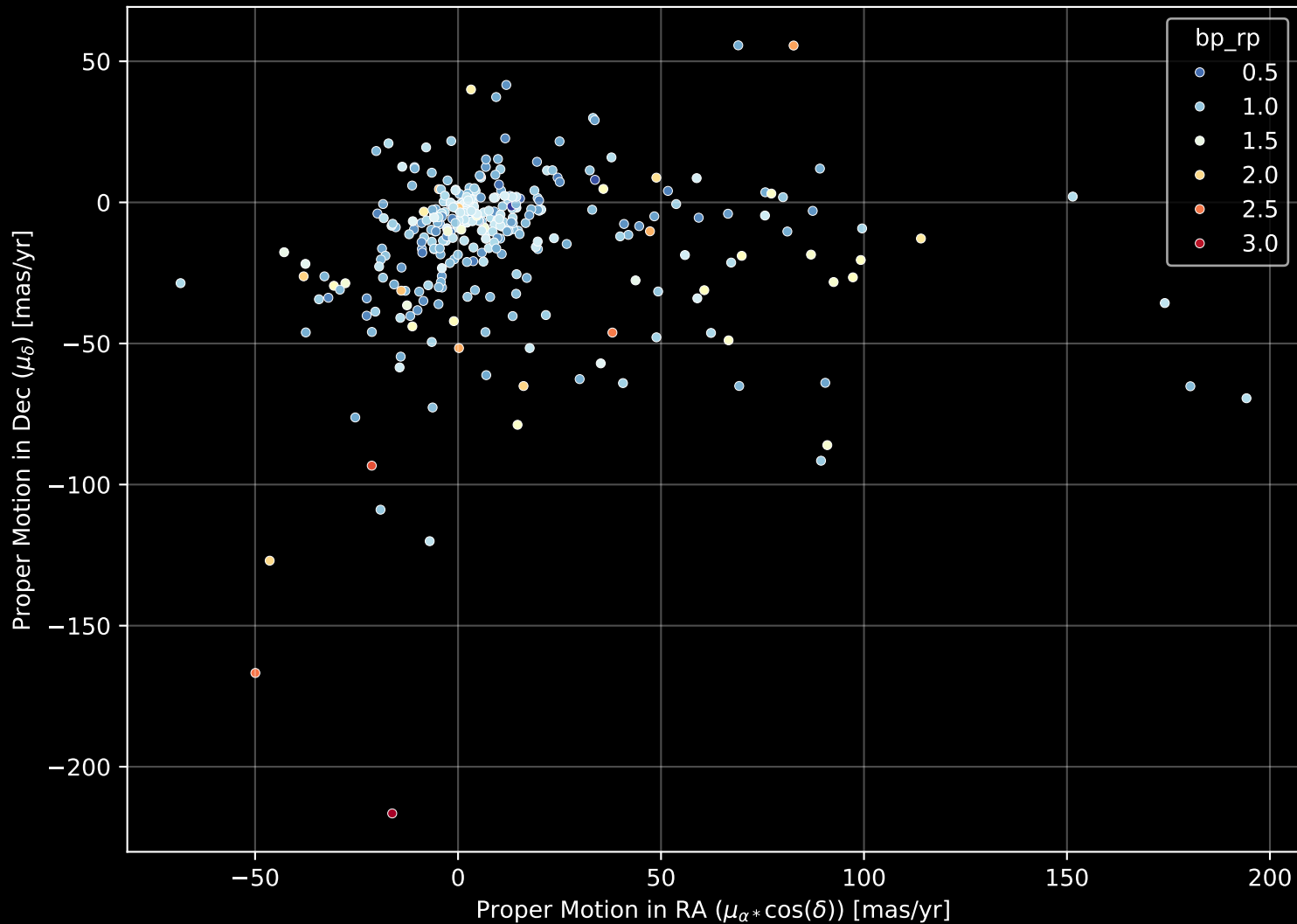
APOGEE DR17 Field: [181-46_MGA] Proper Motion Diagram (n= 326)
