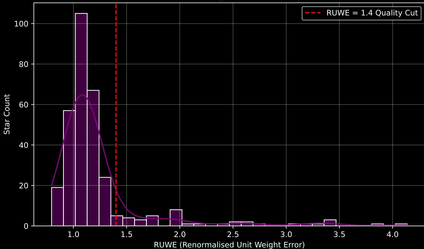
GAPOGEE DR17 Field [181-46_MGA] RUWE Distribution (n= 313)
