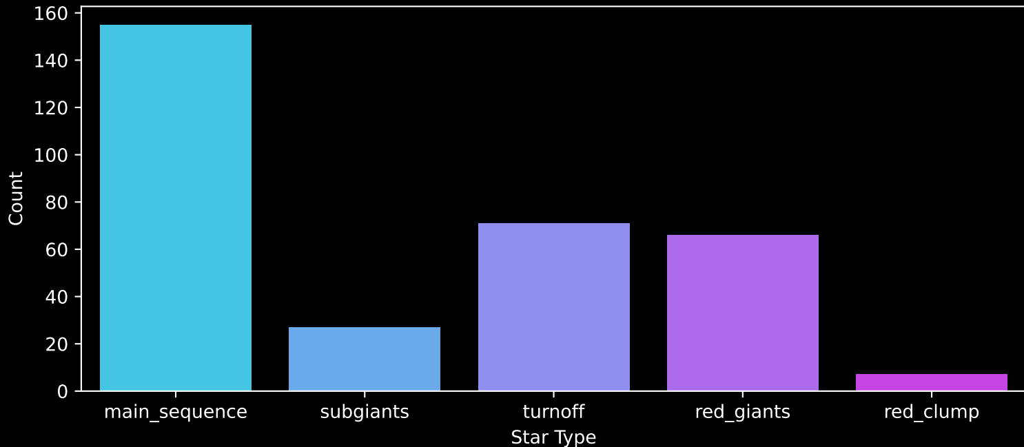
APOGEE DR17 Field: [181-46_MGA] Count plot of Star Type
